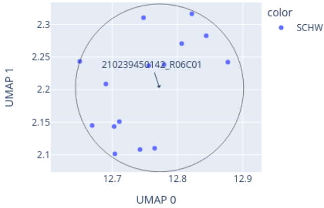
Close-up of UMAP for 210239450142_R06C01 reference: AllIDATv2_20210804_HPAP_Sarc.xlsx (19967 cases), 0 CpGs
