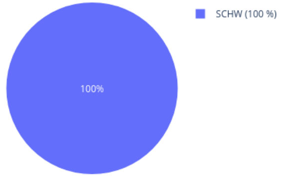
Neighbors in UMAP for 210239450142_R06C01 reference: AllIDATv2_20210804_HPAP_Sarc.xlsx (19967 cases), 0 CpGs
