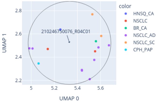
Close-up of UMAP for 210246750076_R04C01 reference: AllIDATv2_20210804_HPAP_Sarc.xlsx (19967 cases), 0 CpGs
