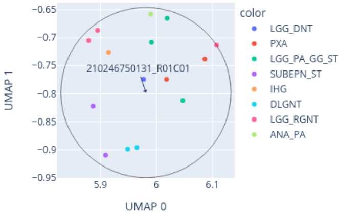
Close-up of UMAP for 210246750131_R01C01 reference: AllIDATv2_20210804_HPAP_Sarc.xlsx (19967 cases), 0 CpGs
