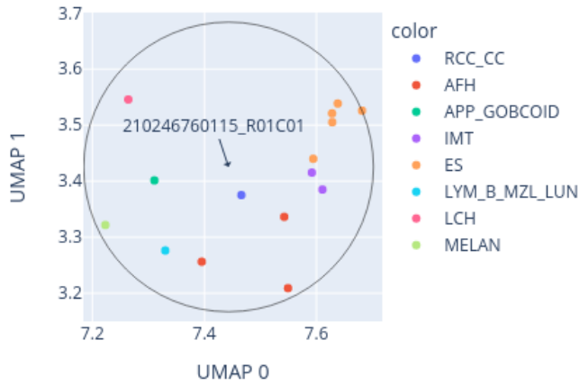
Close-up of UMAP for 210246760115_R01C01 reference: AllIDATv2_20210804_HPAP_Sarc.xlsx (19967 cases), 0 CpGs
