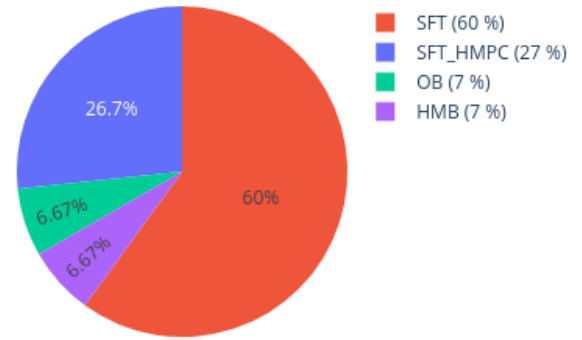
Neighbors in UMAP for 210246760129_R02C01 reference: AllIDATv2_20210804_HPAP_Sarc.xlsx (19967 cases), 0 CpGs
