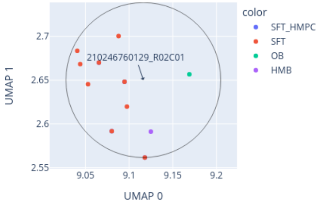
Close-up of UMAP for 210246760129_R02C01 reference: AllIDATv2_20210804_HPAP_Sarc.xlsx (19967 cases), 0 CpGs
