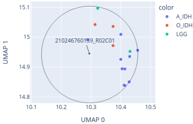
Close-up of UMAP for 210246760139_R02C01 reference: AllIDATv2_20210804_HPAP_Sarc.xlsx (19967 cases), 0 CpGs
