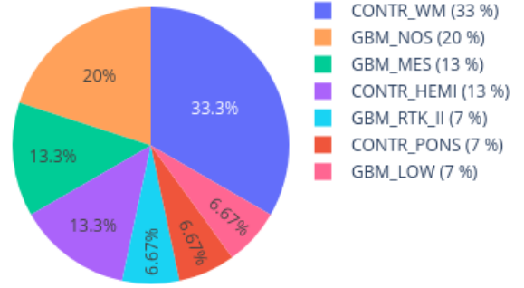
Neighbors in UMAP for 210252210102_R01C01 reference: AllIDATv2_20210804_HPAP_Sarc.xlsx (19967 cases), 0 CpGs
