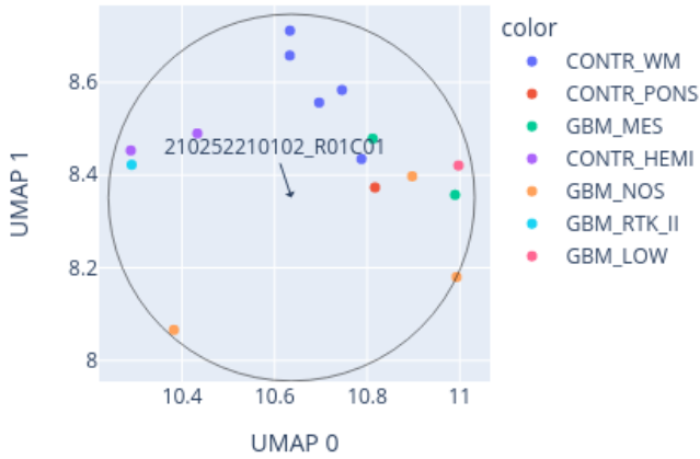
Close-up of UMAP for 210252210102_R01C01 reference: AllIDATv2_20210804_HPAP_Sarc.xlsx (19967 cases), 0 CpGs
