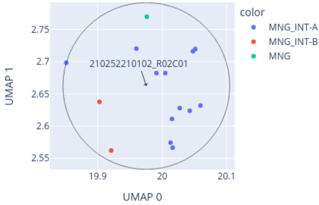
Close-up of UMAP for 210252210102_R02C01 reference: AllIDATv2_20210804_HPAP_Sarc.xlsx (19967 cases), 0 CpGs
