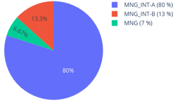
Neighbors in UMAP for 210252210102_R02C01 reference: AllIDATv2_20210804_HPAP_Sarc.xlsx (19967 cases), 0 CpGs
