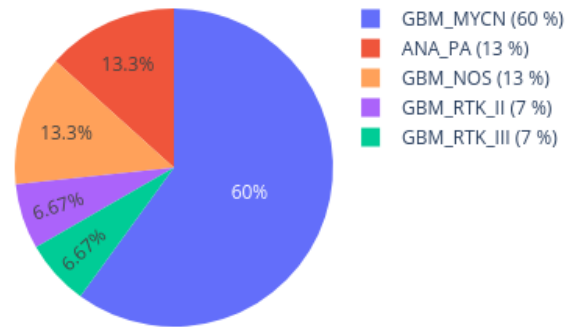
Neighbors in UMAP for 210255220003_R05C01 reference: AllIDATv2_20210804_HPAP_Sarc.xlsx (19967 cases), 0 CpGs
