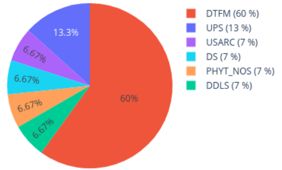
Neighbors in UMAP for 210255220009_R08C01 reference: AllIDATv2_20210804_HPAP_Sarc.xlsx (19967 cases), 0 CpGs
