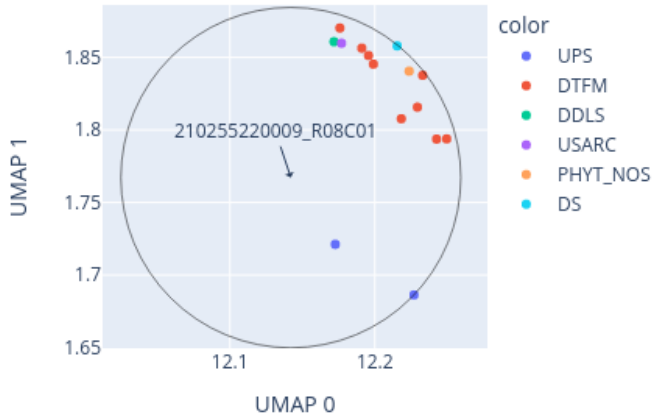
Close-up of UMAP for 210255220009_R08C01 reference: AllIDATv2_20210804_HPAP_Sarc.xlsx (19967 cases), 0 CpGs
