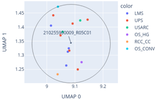
Close-up of UMAP for 210255900009_R05C01 reference: AllIDATv2_20210804_HPAP_Sarc.xlsx (19967 cases), 0 CpGs
