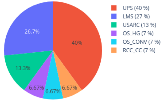
Neighbors in UMAP for 210255900009_R05C01 reference: AllIDATv2_20210804_HPAP_Sarc.xlsx (19967 cases), 0 CpGs
