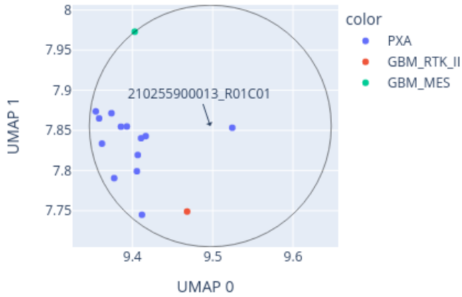
Close-up of UMAP for 210255900013_R01C01 reference: AllIDATv2_20210804_HPAP_Sarc.xlsx (19967 cases), 0 CpGs
