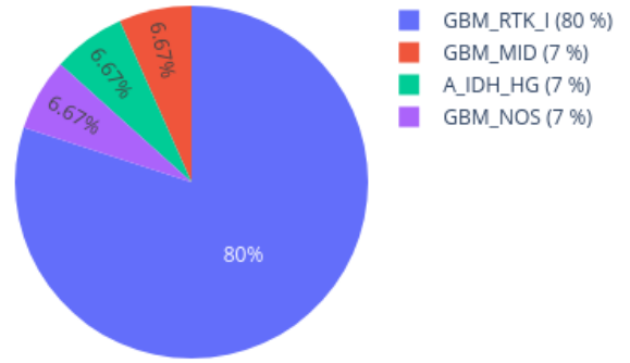
Neighbors in UMAP for 210255900013_R08C01 reference: AllIDATv2_20210804_HPAP_Sarc.xlsx (19967 cases), 0 CpGs
