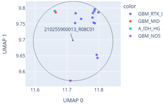
Close-up of UMAP for 210255900013_R08C01 reference: AllIDATv2_20210804_HPAP_Sarc.xlsx (19967 cases), 0 CpGs
