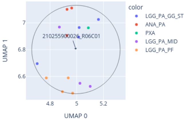
Close-up of UMAP for 210255900026_R06C01 reference: AllIDATv2_20210804_HPAP_Sarc.xlsx (19967 cases), 0 CpGs
