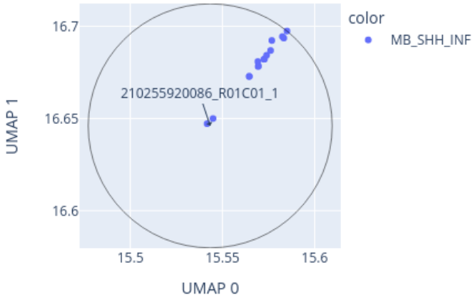
Close-up of UMAP for 210255920086_R01C01_1 reference: AllIDATv2_20210804_HPAP_Sarc.xlsx (19967 cases), 0 CpGs
