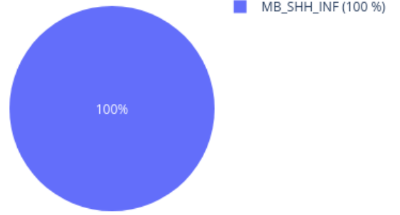
Neighbors in UMAP for 210255920086_R01C01_1 reference: AllIDATv2_20210804_HPAP_Sarc.xlsx (19967 cases), 0 CpGs
