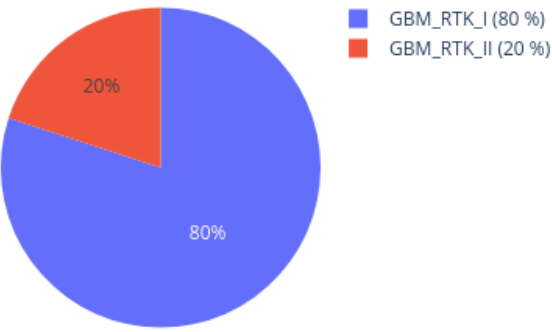
Neighbors in UMAP for 210625920067_R08C01 reference: AllIDATv2_20210804_HPAP_Sarc.xlsx (19967 cases), 0 CpGs
