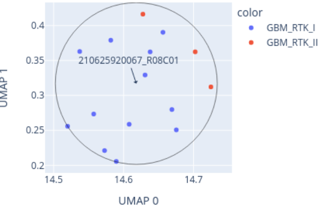
Close-up of UMAP for 210625920067_R08C01 reference: AllIDATv2_20210804_HPAP_Sarc.xlsx (19967 cases), 0 CpGs
