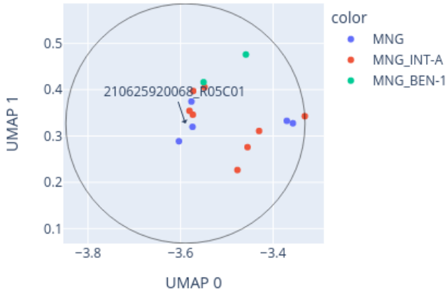
Close-up of UMAP for 210625920068_R05C01 reference: AllIDATv2_20210804_HPAP_Sarc.xlsx (19967 cases), 0 CpGs
