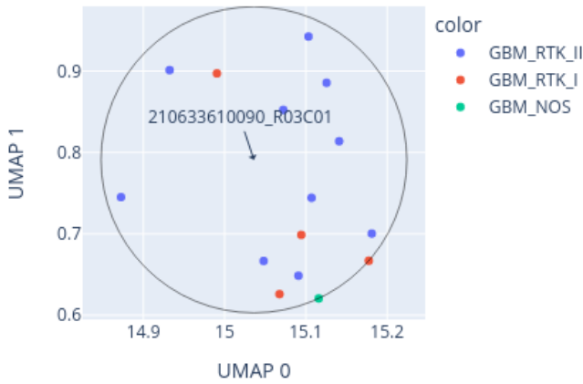
Close-up of UMAP for 210633610090_R03C01 reference: AllIDATv2_20210804_HPAP_Sarc.xlsx (19967 cases), 0 CpGs
