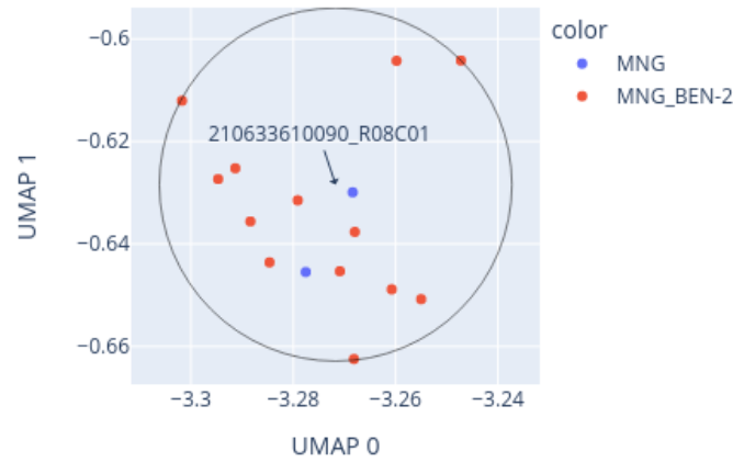
Close-up of UMAP for 210633610090_R08C01 reference: AllIDATv2_20210804_HPAP_Sarc.xlsx (19967 cases), 0 CpGs
