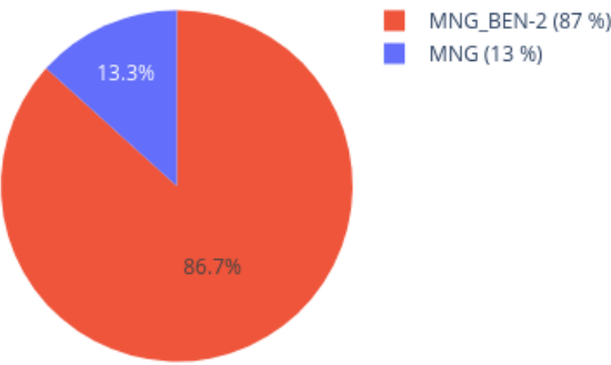
Neighbors in UMAP for 210633610090_R08C01 reference: AllIDATv2_20210804_HPAP_Sarc.xlsx (19967 cases), 0 CpGs
