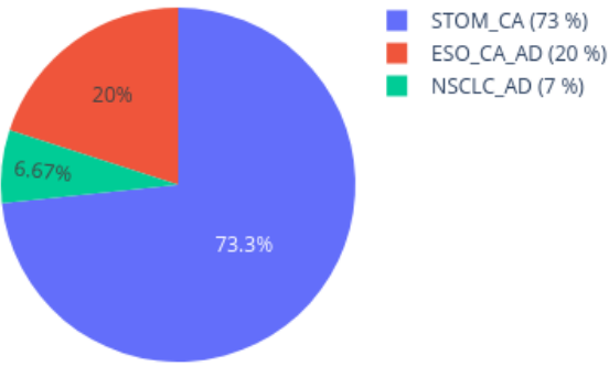
Neighbors in UMAP for 210635130086_R02C01 reference: AllIDATv2_20210804_HPAP_Sarc.xlsx (19967 cases), 0 CpGs
