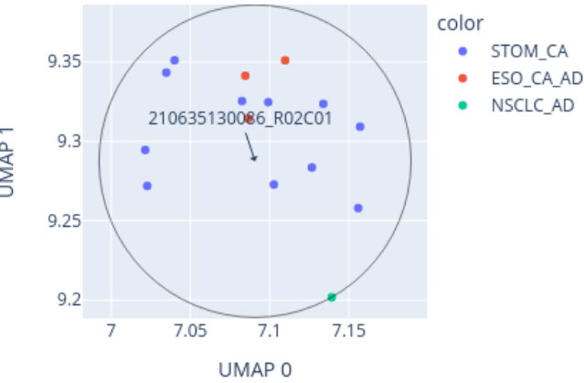
Close-up of UMAP for 210635130086_R02C01 reference: AllIDATv2_20210804_HPAP_Sarc.xlsx (19967 cases), 0 CpGs
