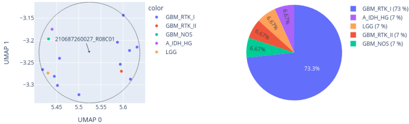
Close-up of UMAP for 210687260027_R08C01 reference: AllIDATv2_20210804_HPAP_Sarc.xlsx (19967 cases), 0 CpGs
