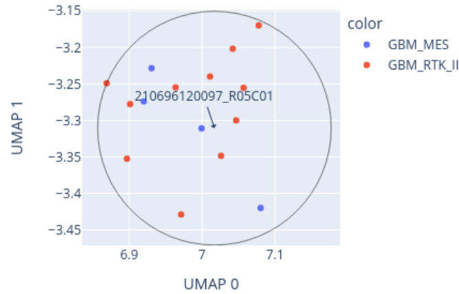
Close-up of UMAP for 210696120097_R05C01 reference: AllIDATv2_20210804_HPAP_Sarc.xlsx (19967 cases), 0 CpGs
