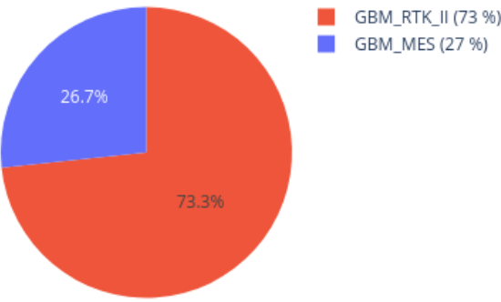
Neighbors in UMAP for 210696120097_R05C01 reference: AllIDATv2_20210804_HPAP_Sarc.xlsx (19967 cases), 0 CpGs
